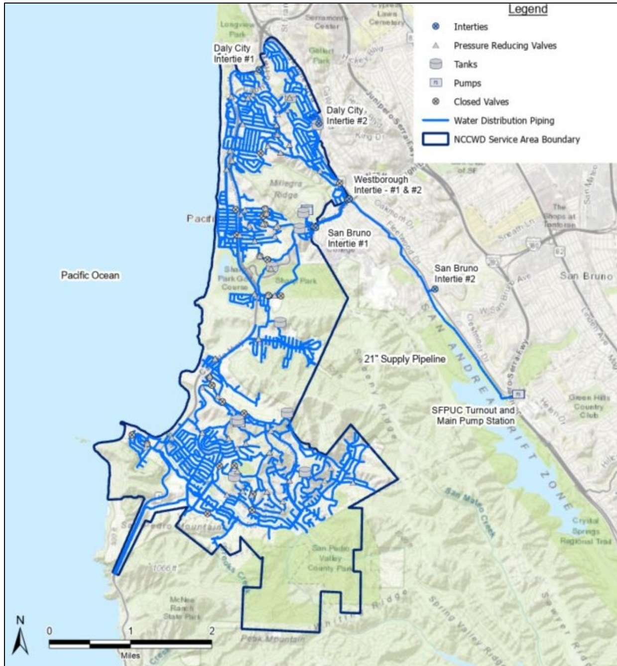
Figure 3-7 District Potable Water Distribution System
