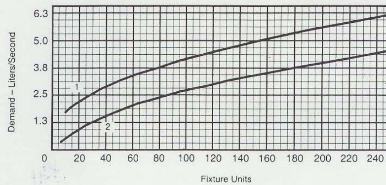
CHART A-3 (Metric) Enlarged Scale Demand Load
